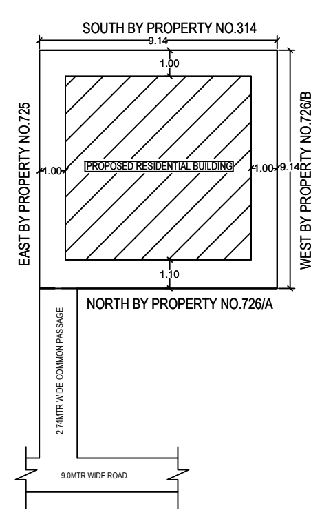
SITE PLAN
